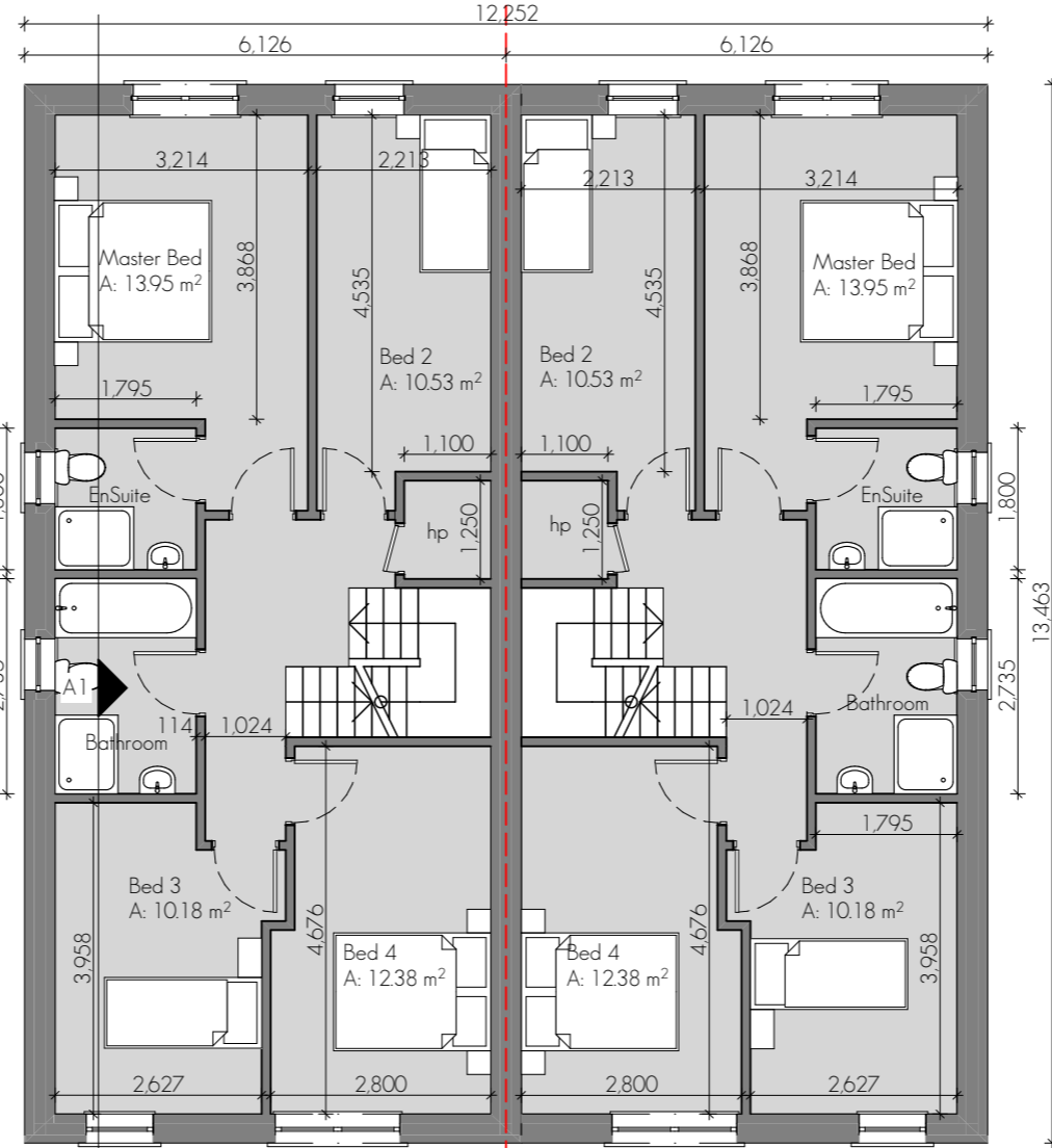
FIRST FLOOR A1/A1 1:100
