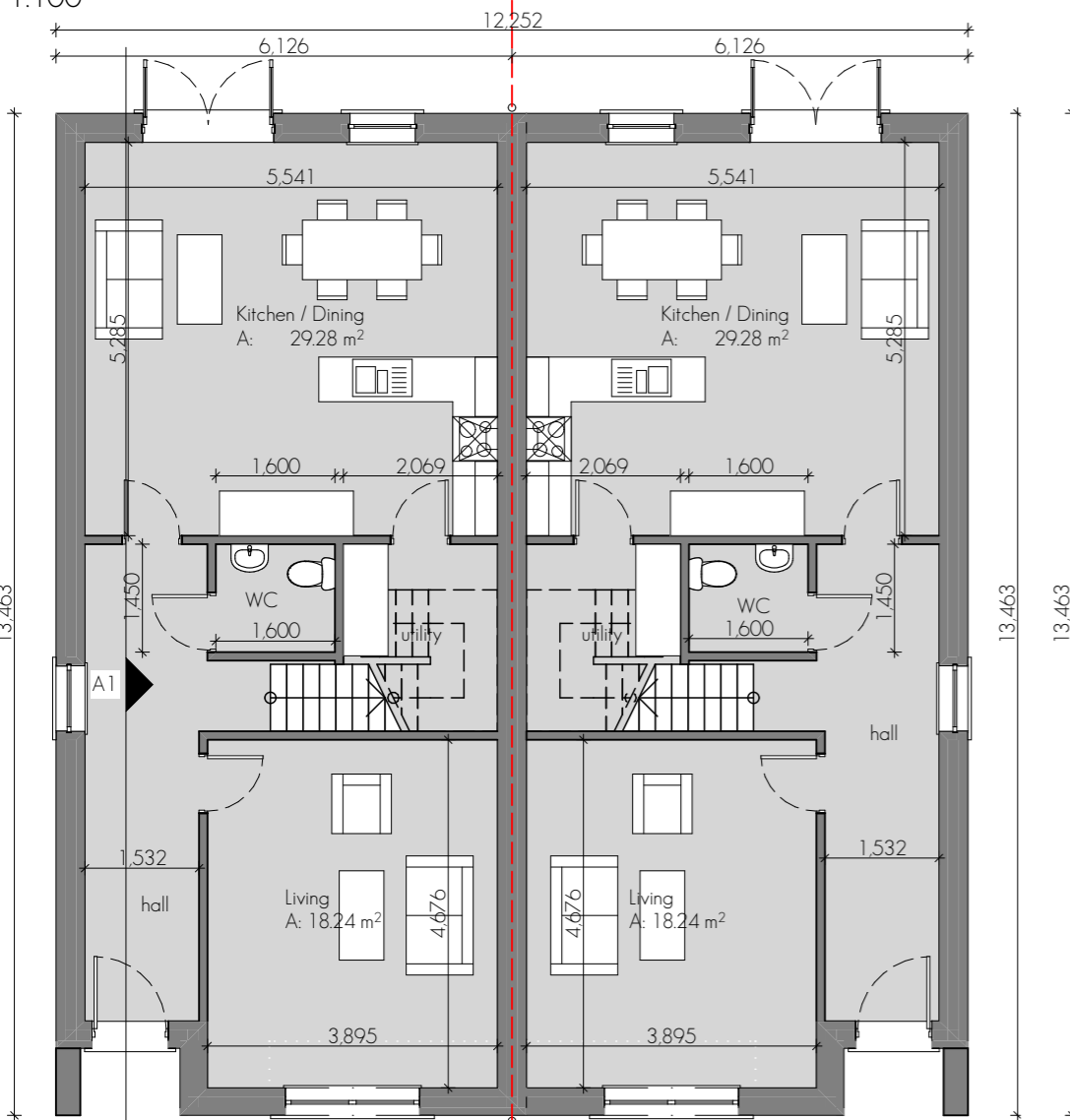
GROUND FLOOR A1/A1 1:100
